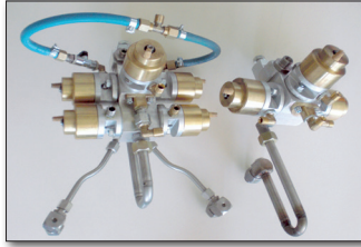
Airless 2-component spray gun and double spray gun M98:2 and M1:1
