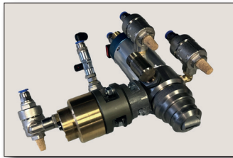
Airspray 2K-Spritzpistole M98:2
